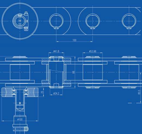
Chain with exterior roller
