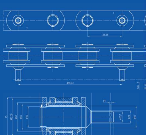
self lubricated chain
