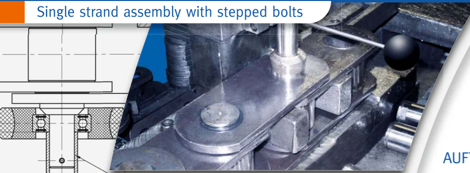
Check and measure the single strand chain
