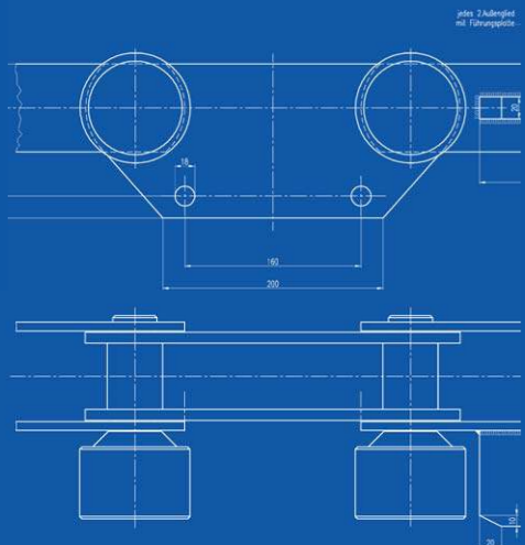
Scraper chain
