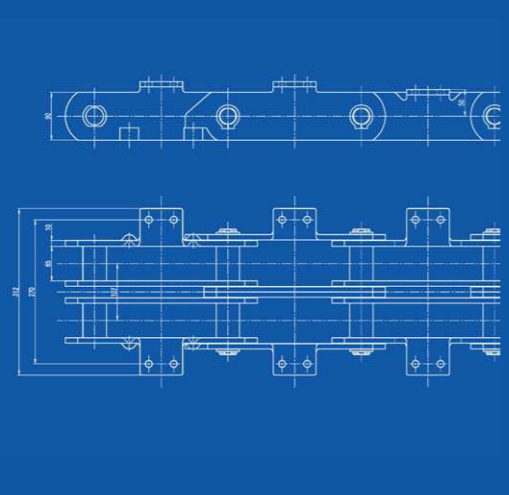
Duplex chain
